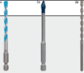
HEX-9 Multi-Construction Ø 6 mm Largo: 66/198 mm HEX-9 Hard Ceramic Ø 6 mm Largo: 99 mm CYL-3 Ø 6 mm Largo: 66/166 mm
